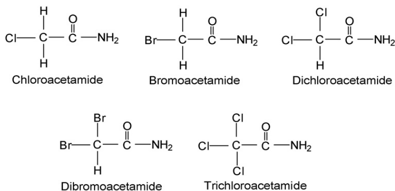
Fig. 3. Structures of haloamides.
