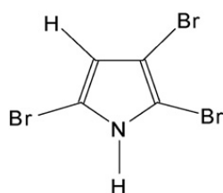
Fig. 4. Structure of 2,3,5-tribromopyrrole.
