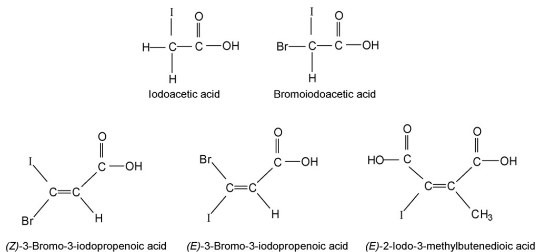
Fig. 1. Structures of iodo-acids.
