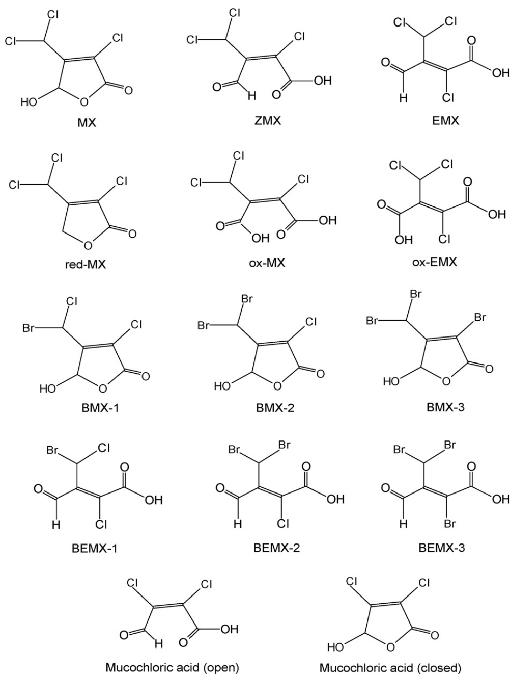
Fig. 2. Structures of MX analogues.
