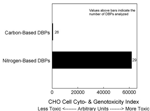
Fig. 8. Combined toxicity index values for carbonaceous DBPs (C-DBPs, i.e., those that do not contain nitrogen) versus nitrogenous DBPs (N-DBPs, i.e., those that contain nitrogen) [62].
