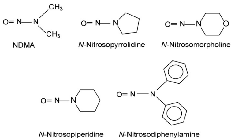
Fig. 5. Structures of NDMA and other nitrosamine DBPs.
